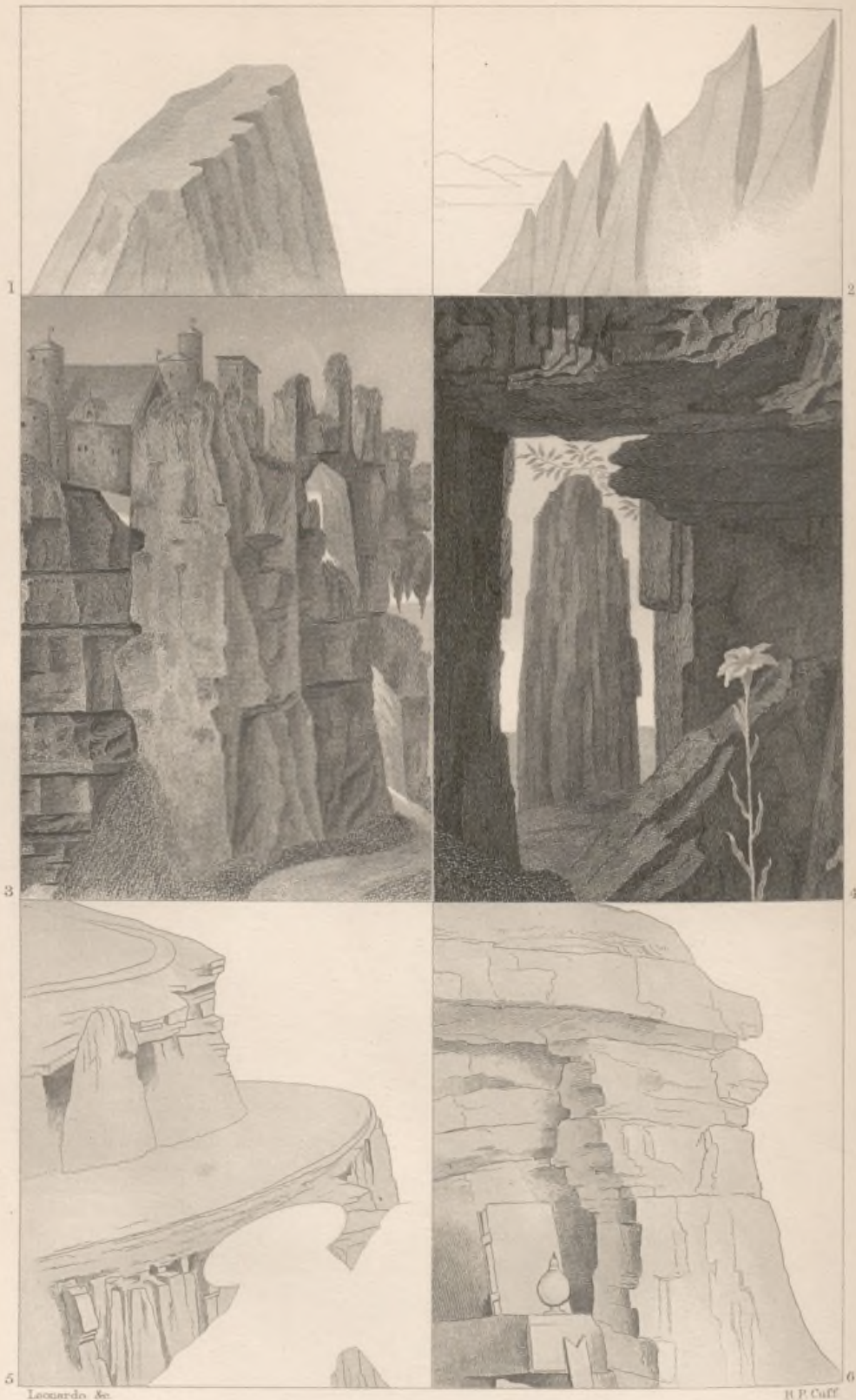
10. Geology of the Middle Ages.
