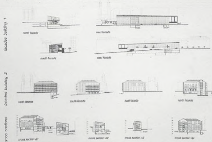
Situation, Facades and Cross sections
